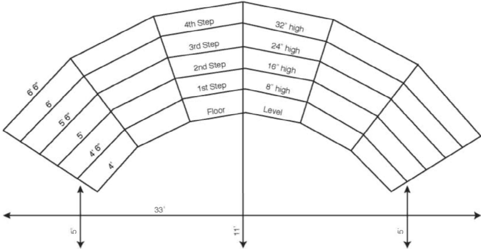
Diagram for 6 - 6" sections of 18" choral risers including 4th step and floor.
